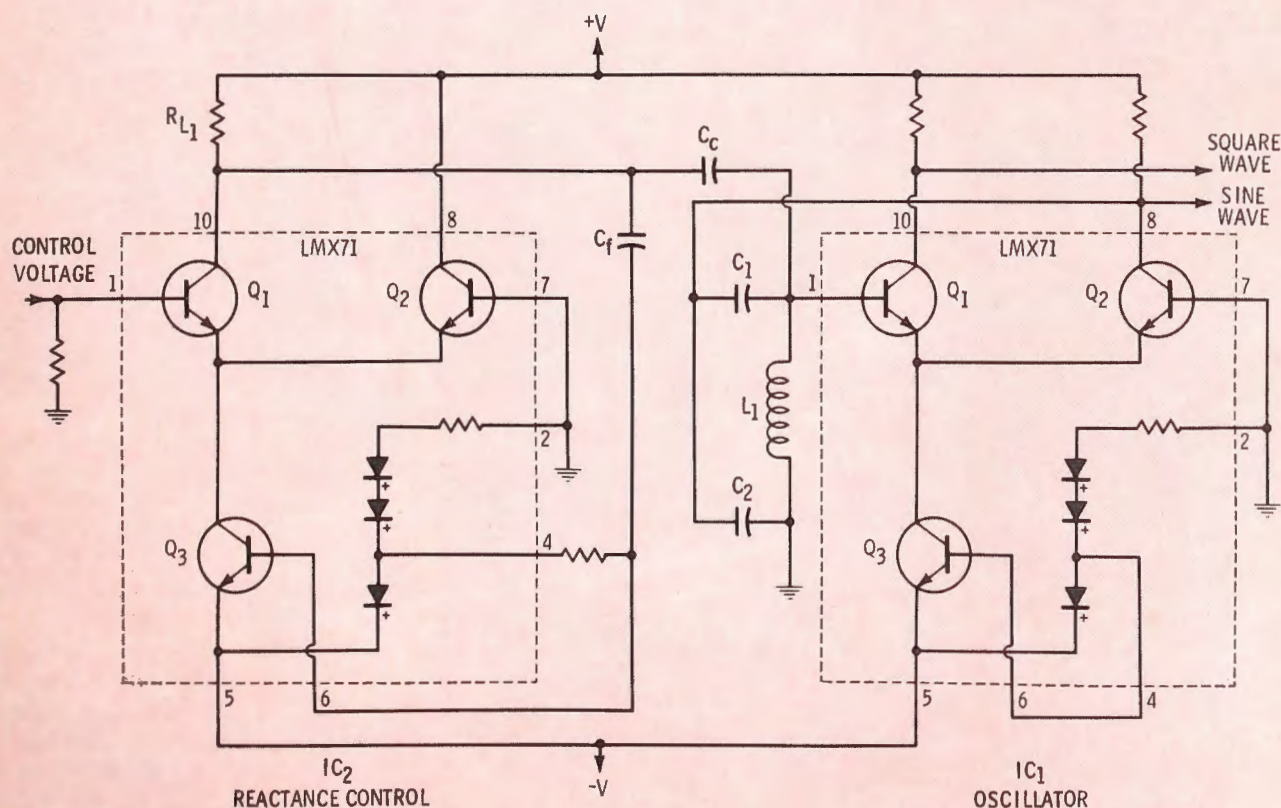
Fig. 3 Voltage controlled oscillator.
