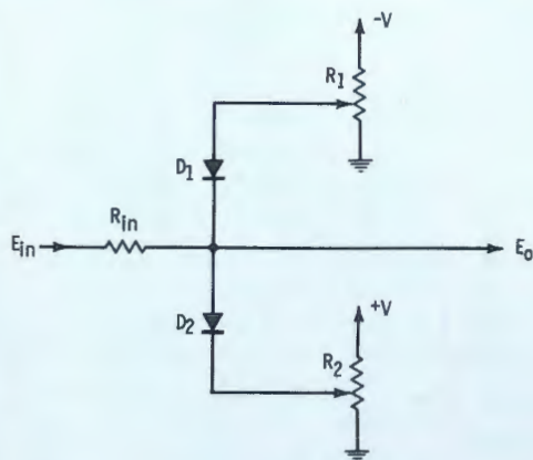
Fig. 9b Simplified clipper.
