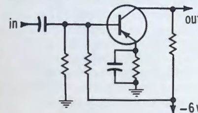
Fig. 1 (C) Base voltage stabilization by a voltage divider. The emitter resistor helps thermal stabilization the most of the two methods.
