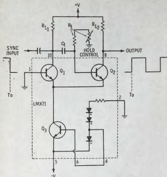
Fig. 6a RC coupled synchronized astable oscillator.
