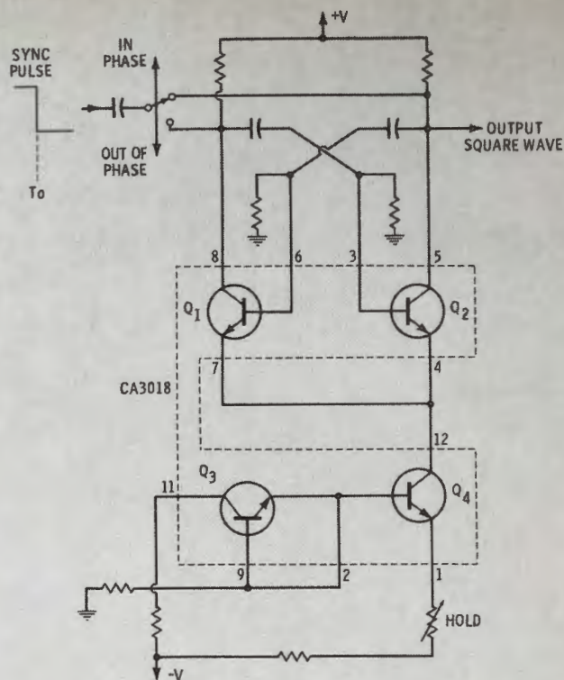
Fig. 6b RC coupled synchronized symmetrical astable oscillator.
